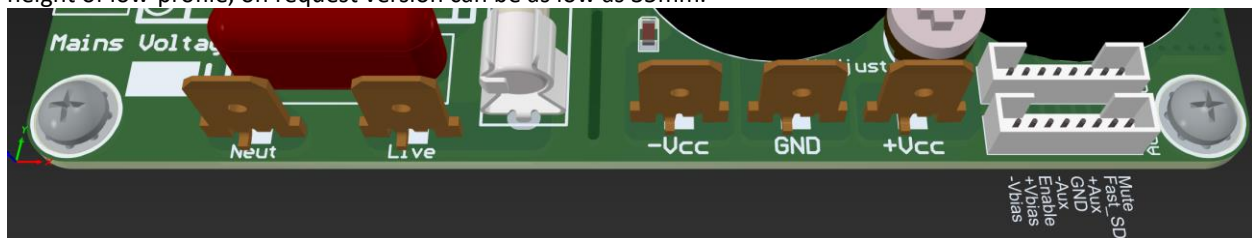
Fig.3 SMPS600RxE board layout and connectors location
