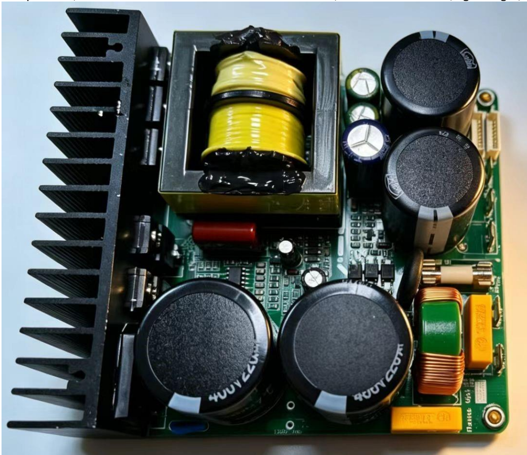
Fig.1 SMPS600RxE appearance
