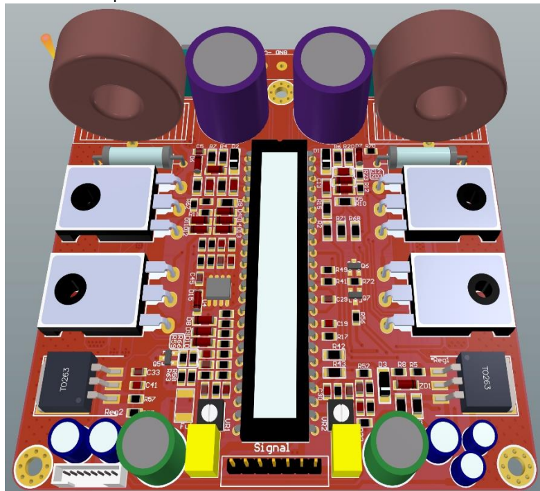
Figure 4: TA3020 Audio Amplifier Module Board layout overview
