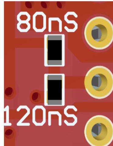
Figure 3: Amplifier BBM Setting
