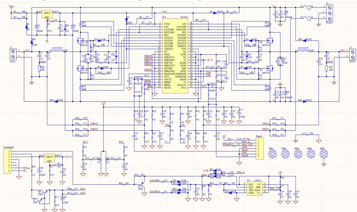
Figure 2: TA3020 v3a Audio Amplifier Module Schematic Diagram
