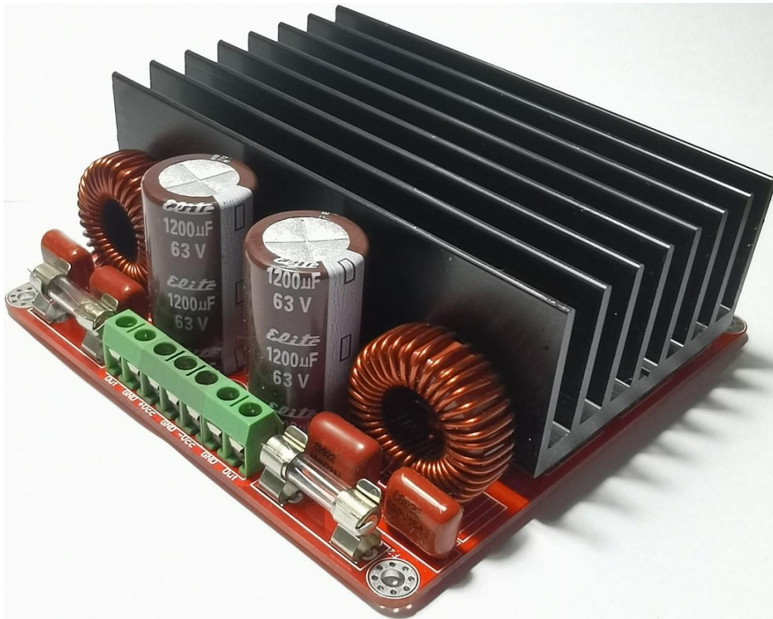
Figure 1: TA3020 Audio Amplifier Module v3.10
