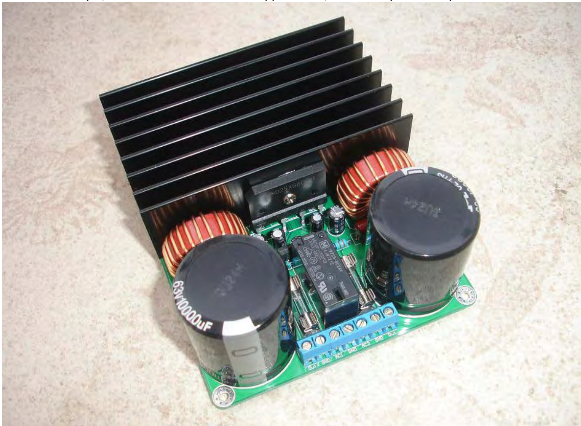
Figure 1: TA3020 Audio Amplifier Module v3c
