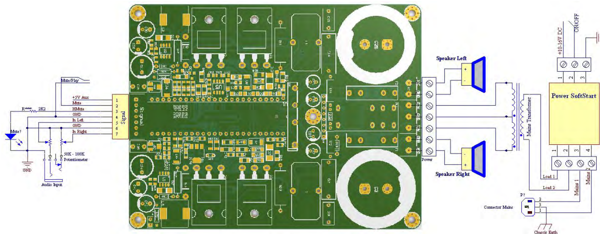
Figure 5: TA3020v3c Amplifier Basic Connection Diagram
