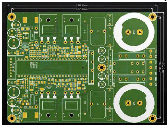
Figure 4: TA3020 Audio Amplifier module Board layout overview and connections
